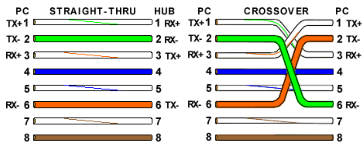
Figure 1.7: Straight through and crossover cable wire scheme
