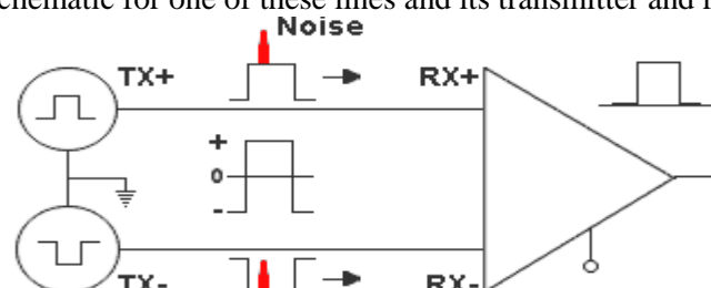
Figure 1.6: Schematic diagram of transmission line
