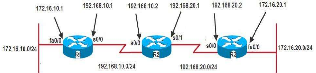
Figure 4.1: Scenario for static routes
