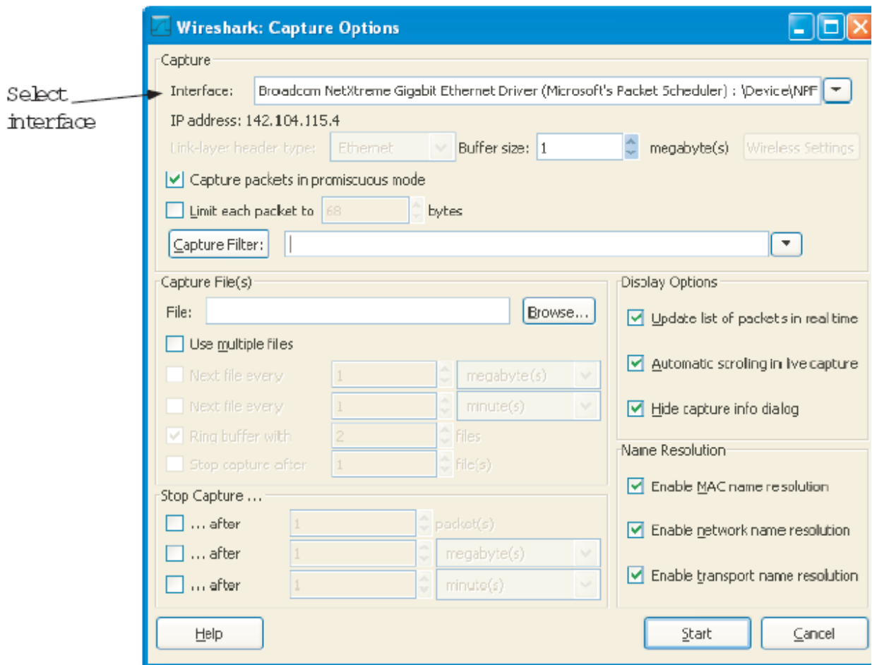
Figure 11.3 Capture options window
