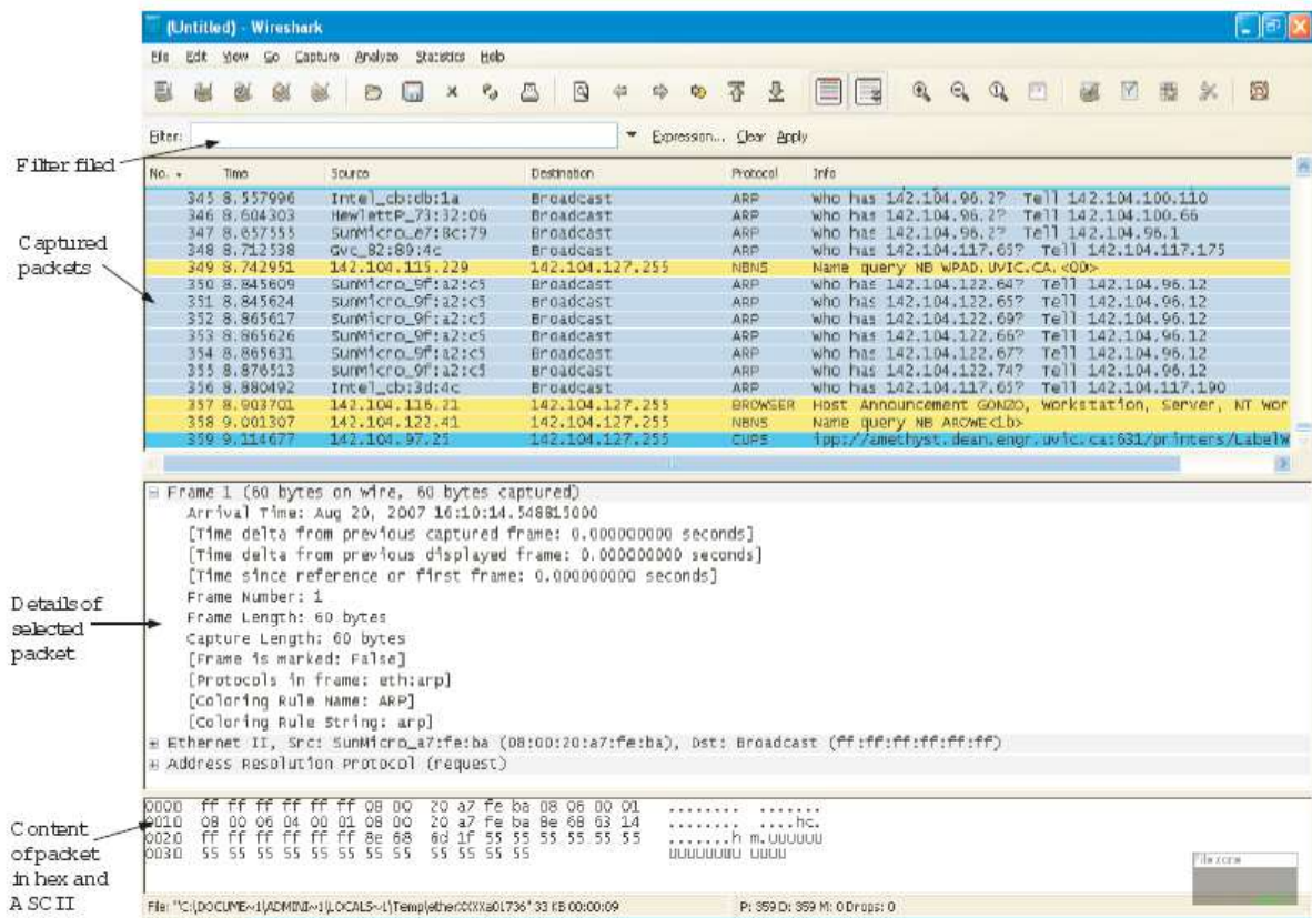
Figure 11.2: WireShark Graphical User Interface
