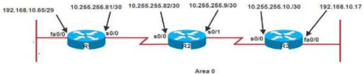
Fig 6.1: Scenario for OSPF implementation
