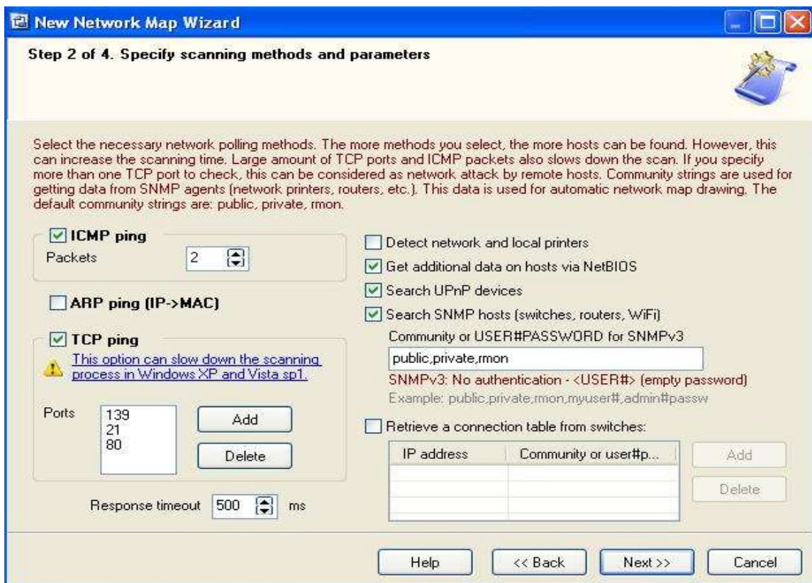
Figure 10.3 Scanning methods and parameters on LANState
