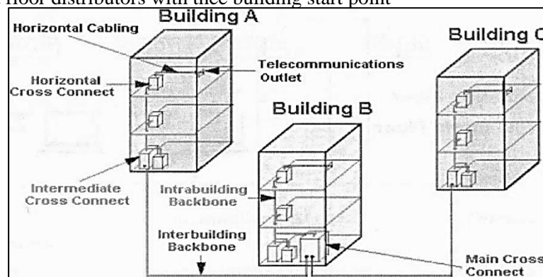
Figure 14.1: building-building connection using fiber optics as backbone
