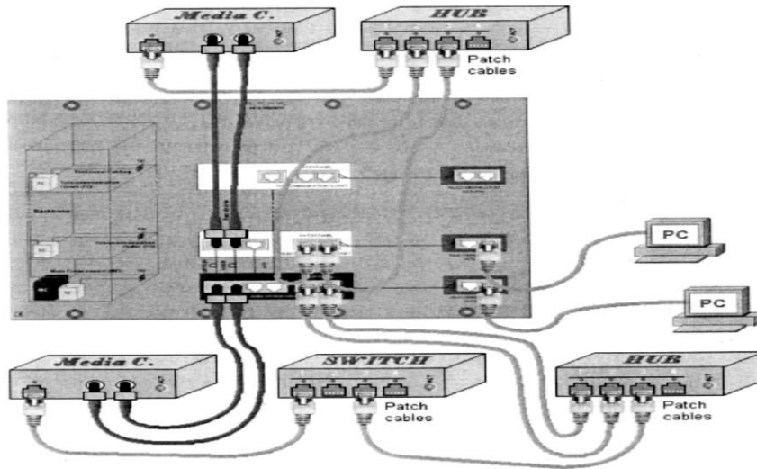
Figure 14.2: connection diagram
